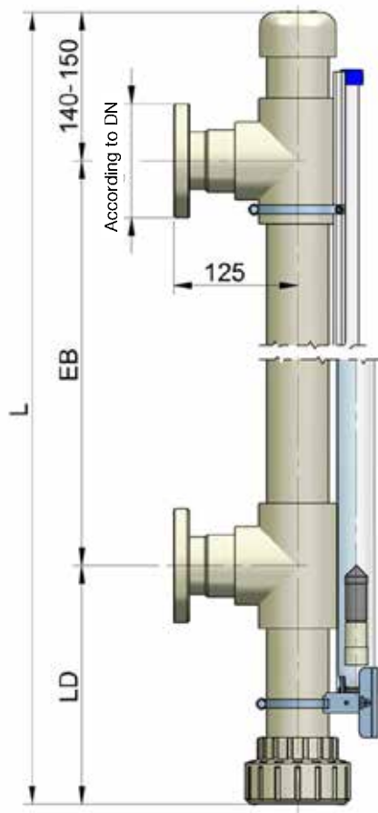
LT ... LTL14 / PP, PVC, PVC-C, PVDF
