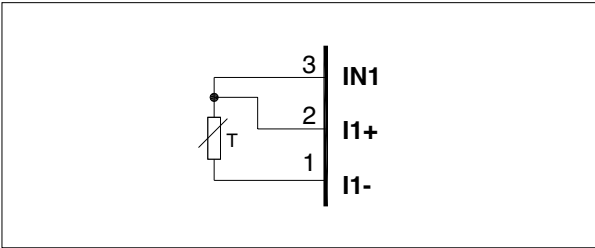
Figure 19 Connection scheme for Pt100 input
