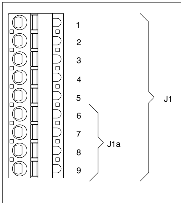
Figure 8 Connector J1
