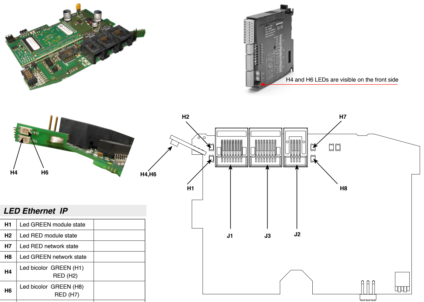
Figure 28 Port2: Modbus RTU / Ethernet IP or Modbus RTU/EtherCAT or Modbus RTU / ProfiNET Interfaces
