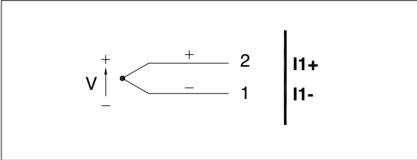
Figure 18 Connection scheme for 60mV TC/linear input
