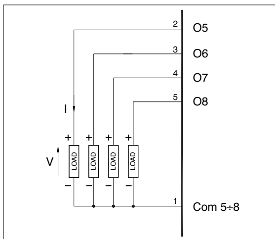
Figure 9 Connection scheme for logic/continuous outputs
