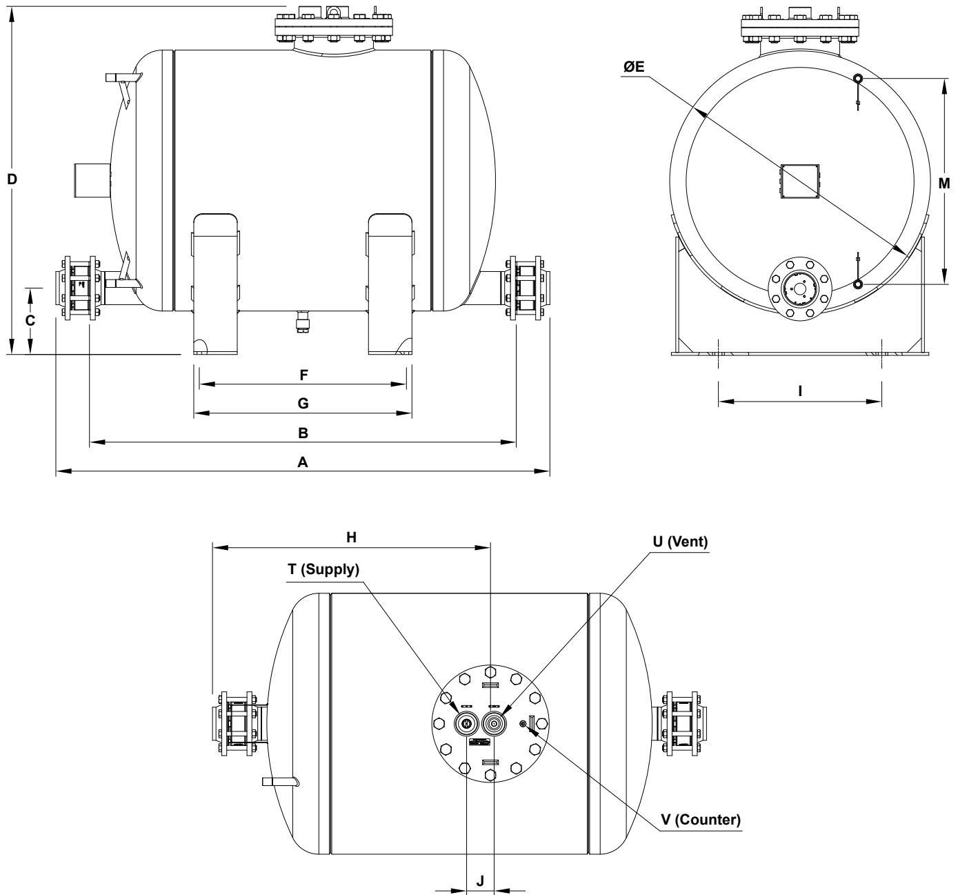
DIMENSIONS (mm)
