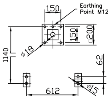
Fixing Detail
