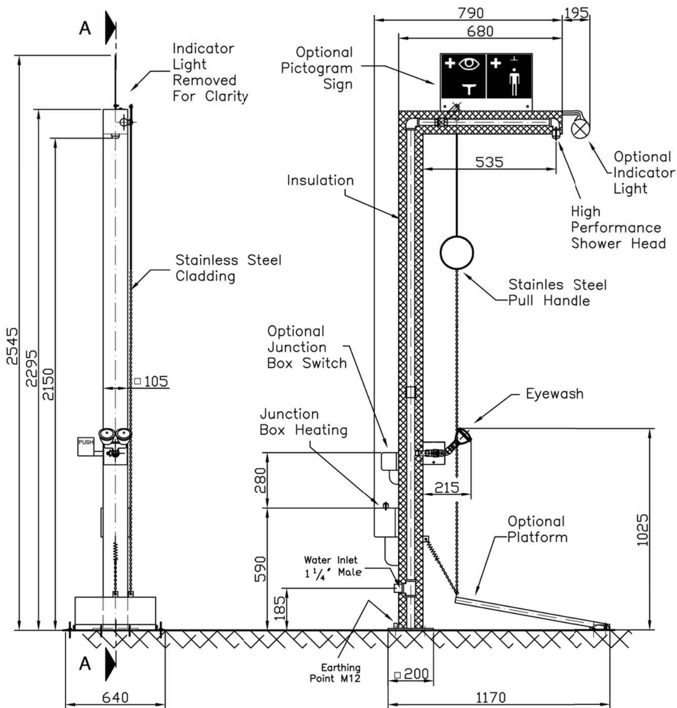
Fixing Detail
