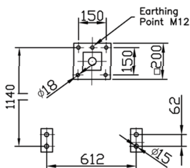
Fixing Detail
