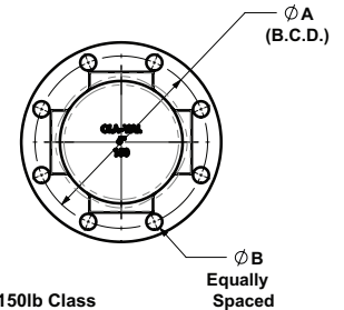
6" Test Header 150lb Class Flat Face Shown
