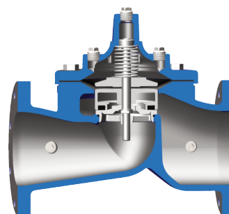
Model 100-20 Reduced Port Hytrol Main Valve
